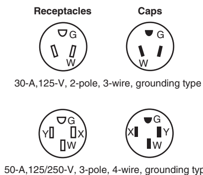
FIGURE 552.44(C)(1) Attachment Cap and Receptacle Configurations.
